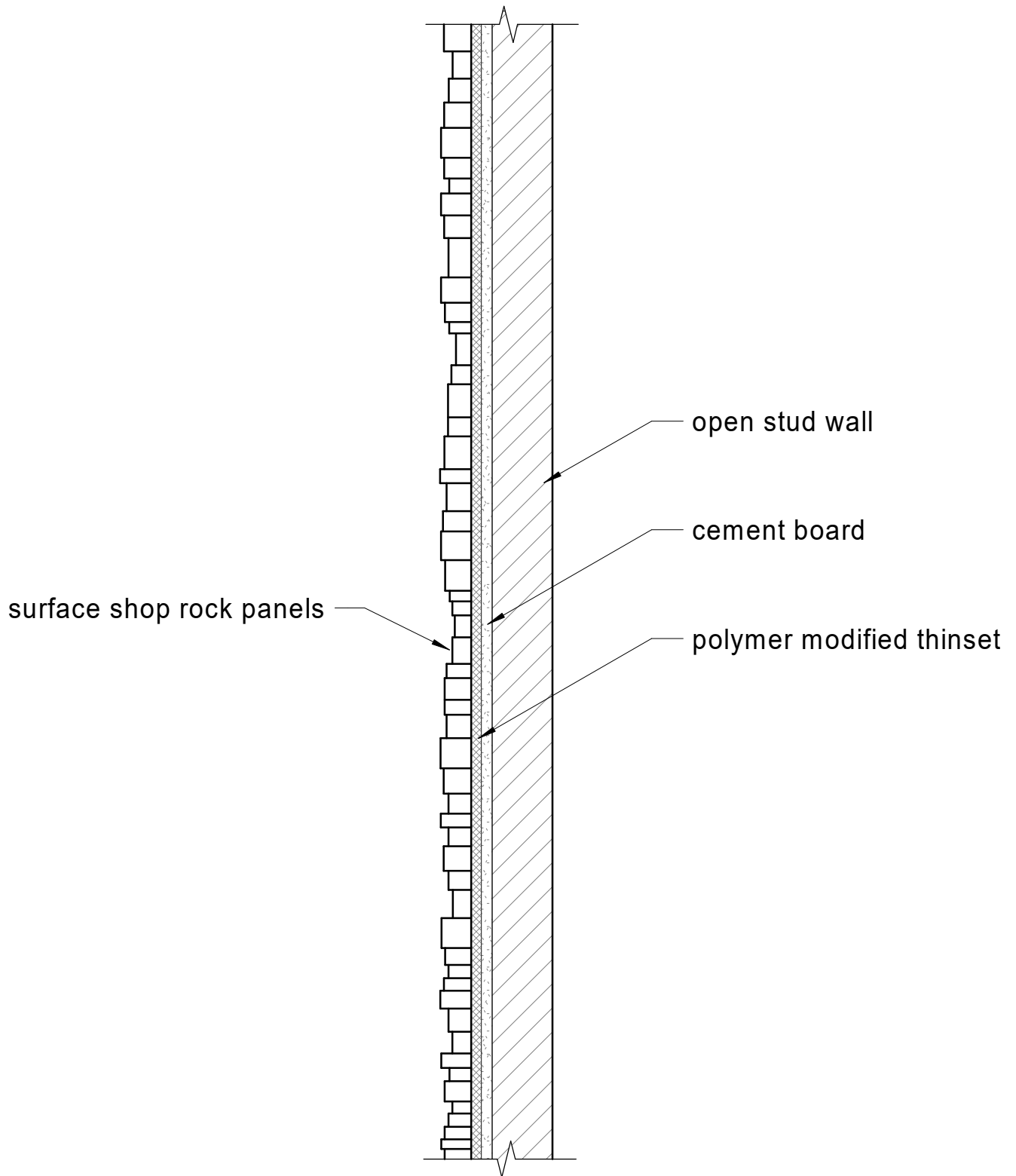
rock panel detail - open stud wall - interior
