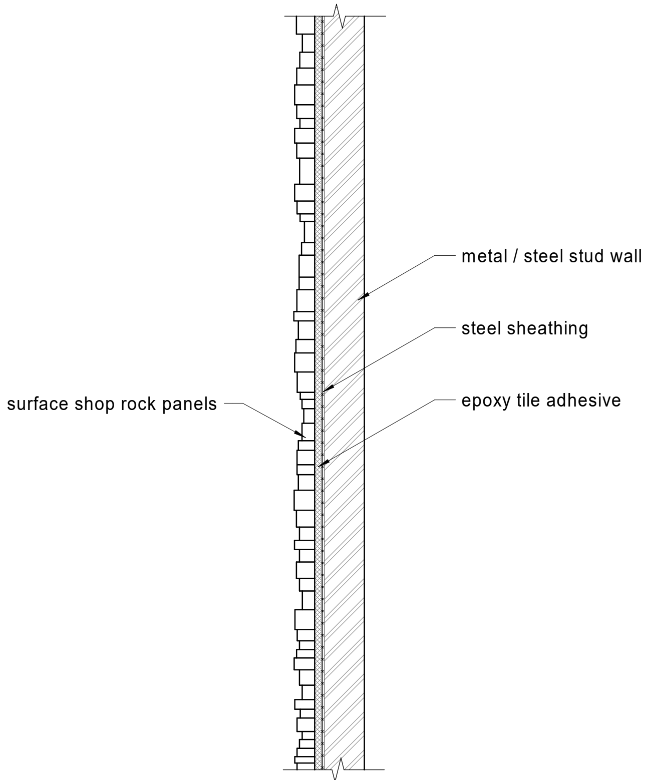
rock panel detail - steel #2 - exterior
